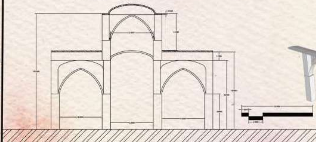
نما Front View
